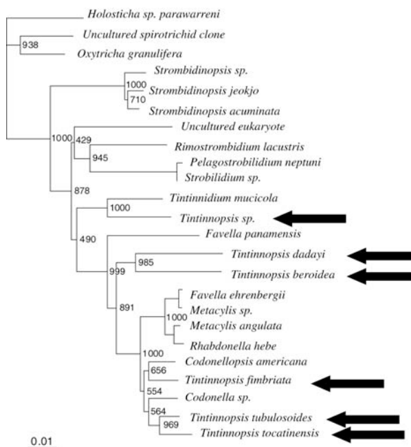
Fig. 1. Neighbor-joining tree from 18S sequences of tintinnids and some other members of the class Spirotrichea available on GenBank. Bootstrap values are based on 1000 iterations. Arrows indicate Tintinnopsis spp., whose positions indicate either a lack of monophyly in the genus or the tendency to misidentify it.
